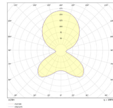
ONO FLUSH MOUNT 350
